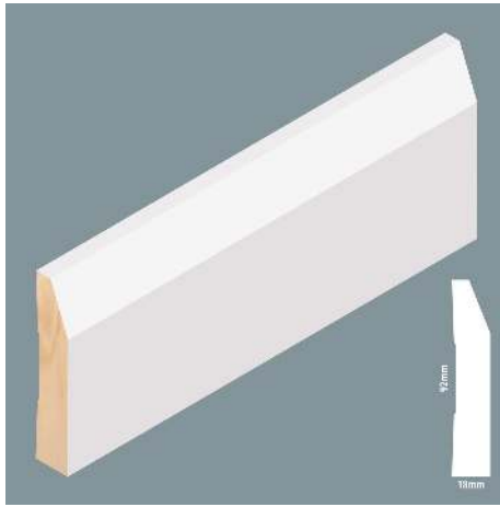
HALF SPLAYED
