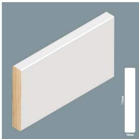
WINDOW REVEALS
