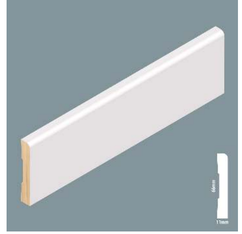
PENCIL ROUND
